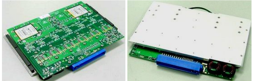
28Vinput, 4 Output, 550W Max VME Card
