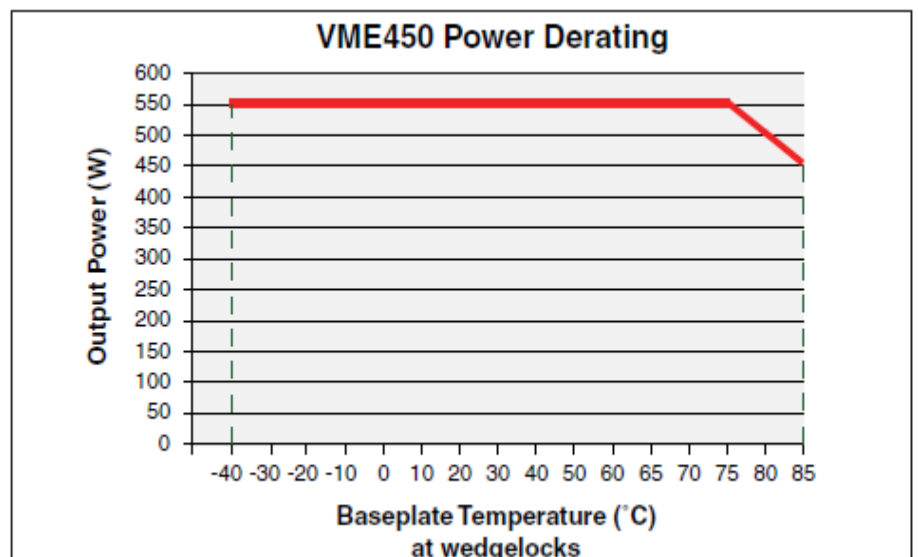
Figure 1. Power Derating
